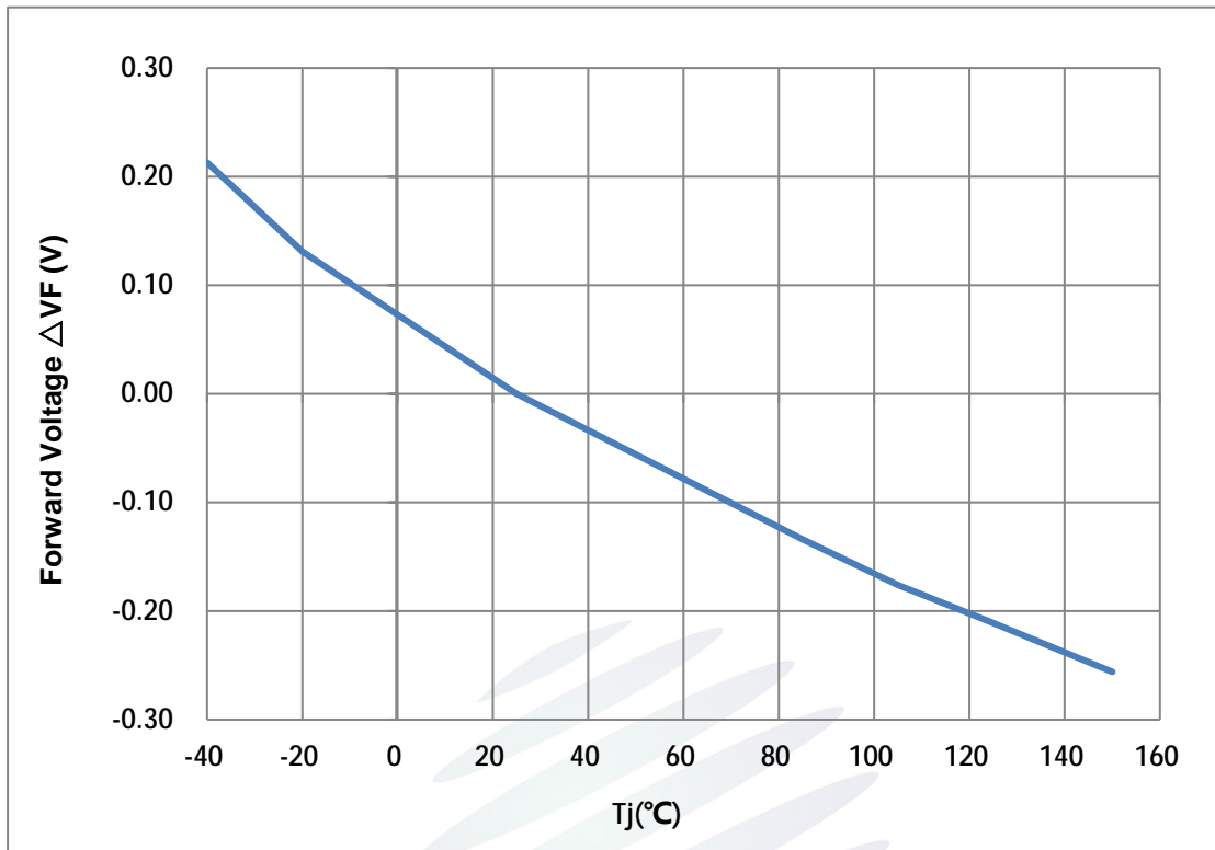
Fig. 1-11 Voltage Shift Vs Junction Temperature
