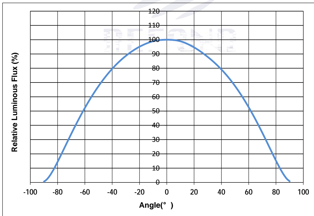
Fig. 1-12 Radiation Diagram
