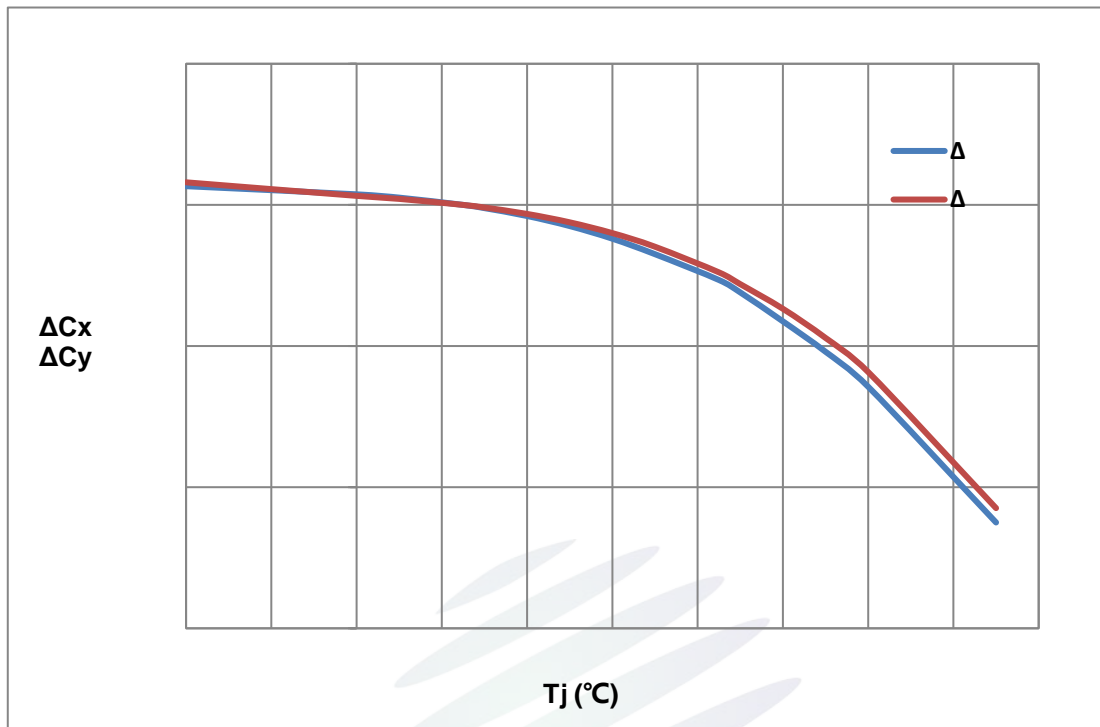
Fig. 1-13 Chromaticity Coordinate Shift Vs Junction Temperature
