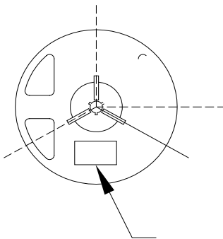
Fig.2-2 Reel Dimension
